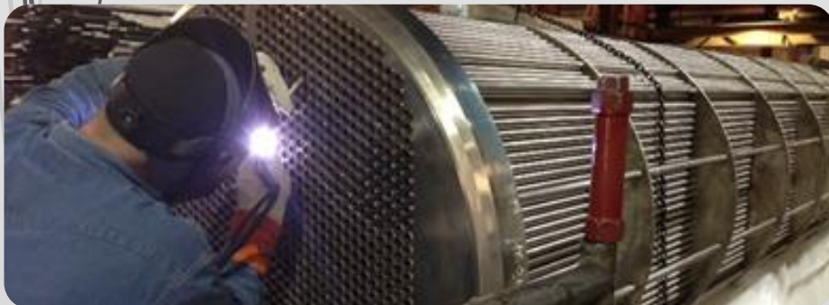
Tube to Tube-sheet Joint welding
